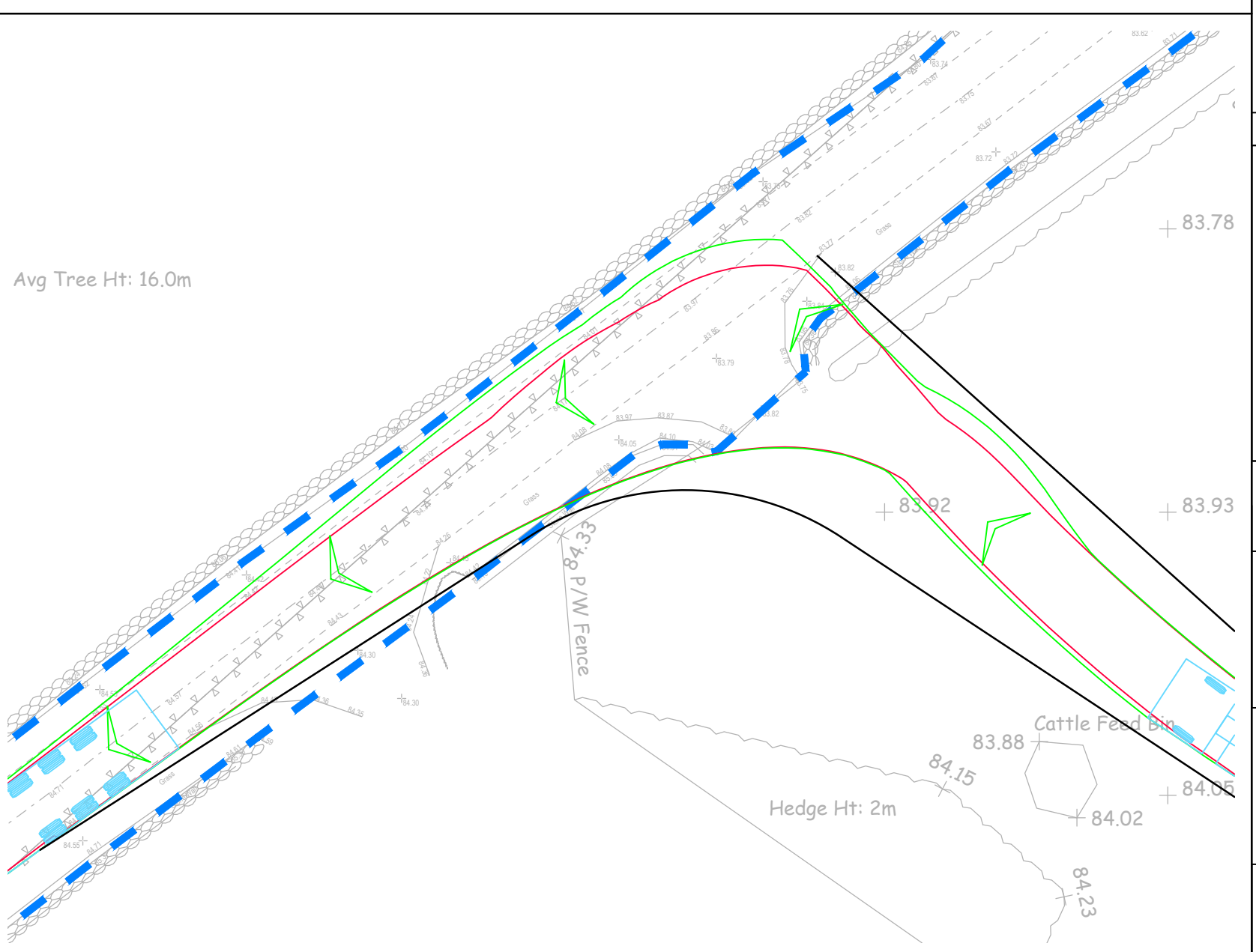
Articulated HGV Turning Left Out Of Access Scale 1:200
