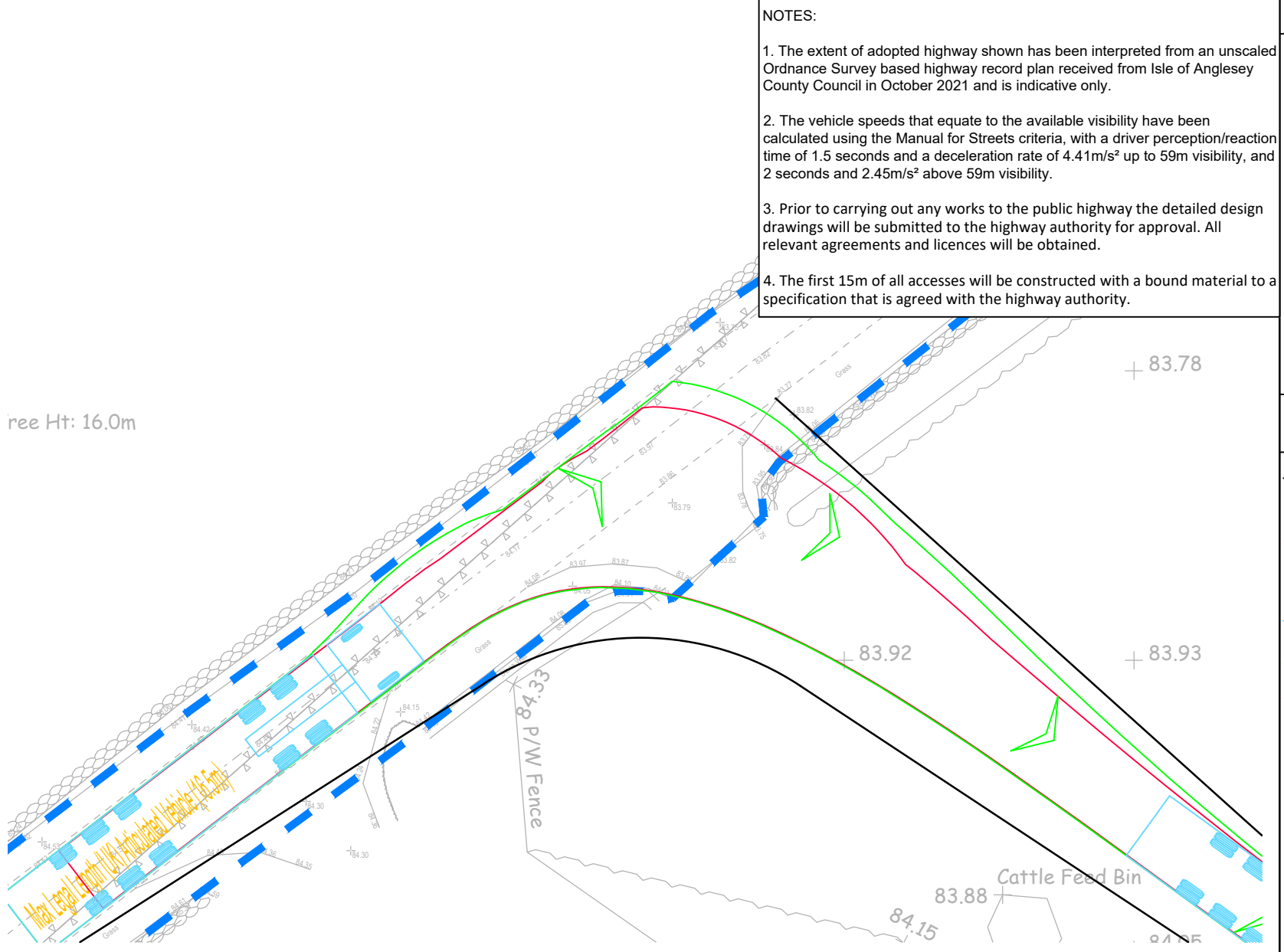
Articulated HGV Turning Right Into Access Scale 1:200
